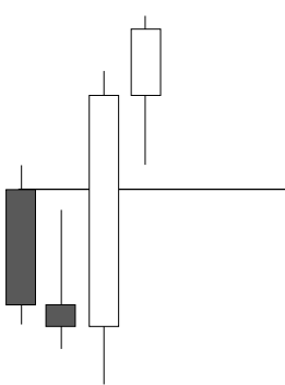
order block
