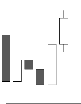
external low
