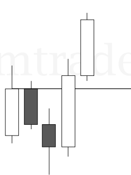
breaker block
