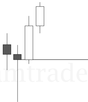
rejection block
