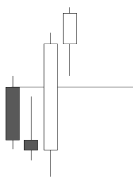
order block
