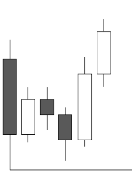
external low
